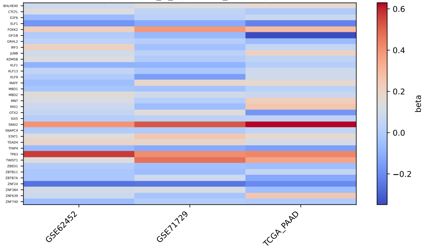
phase9b1_tf_replication_heatmap
