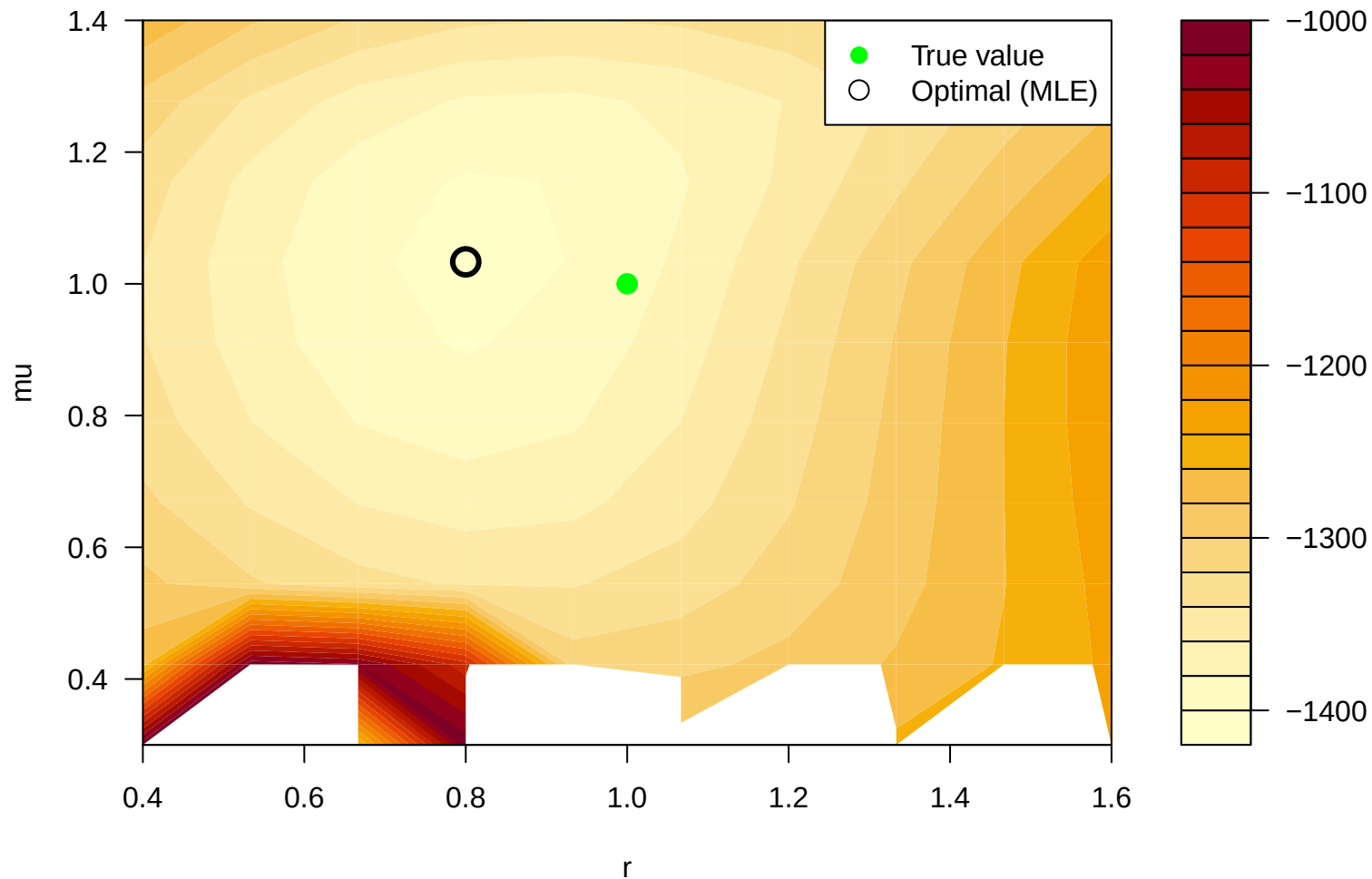
Likelihood surface, in the mu vs. r plane, ekf
