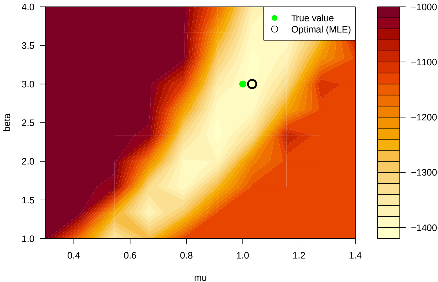
Likelihood surface, in the beta vs. mu plane, laplace
