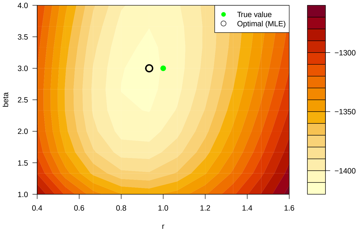
Likelihood surface, in the beta vs. r plane, laplace
