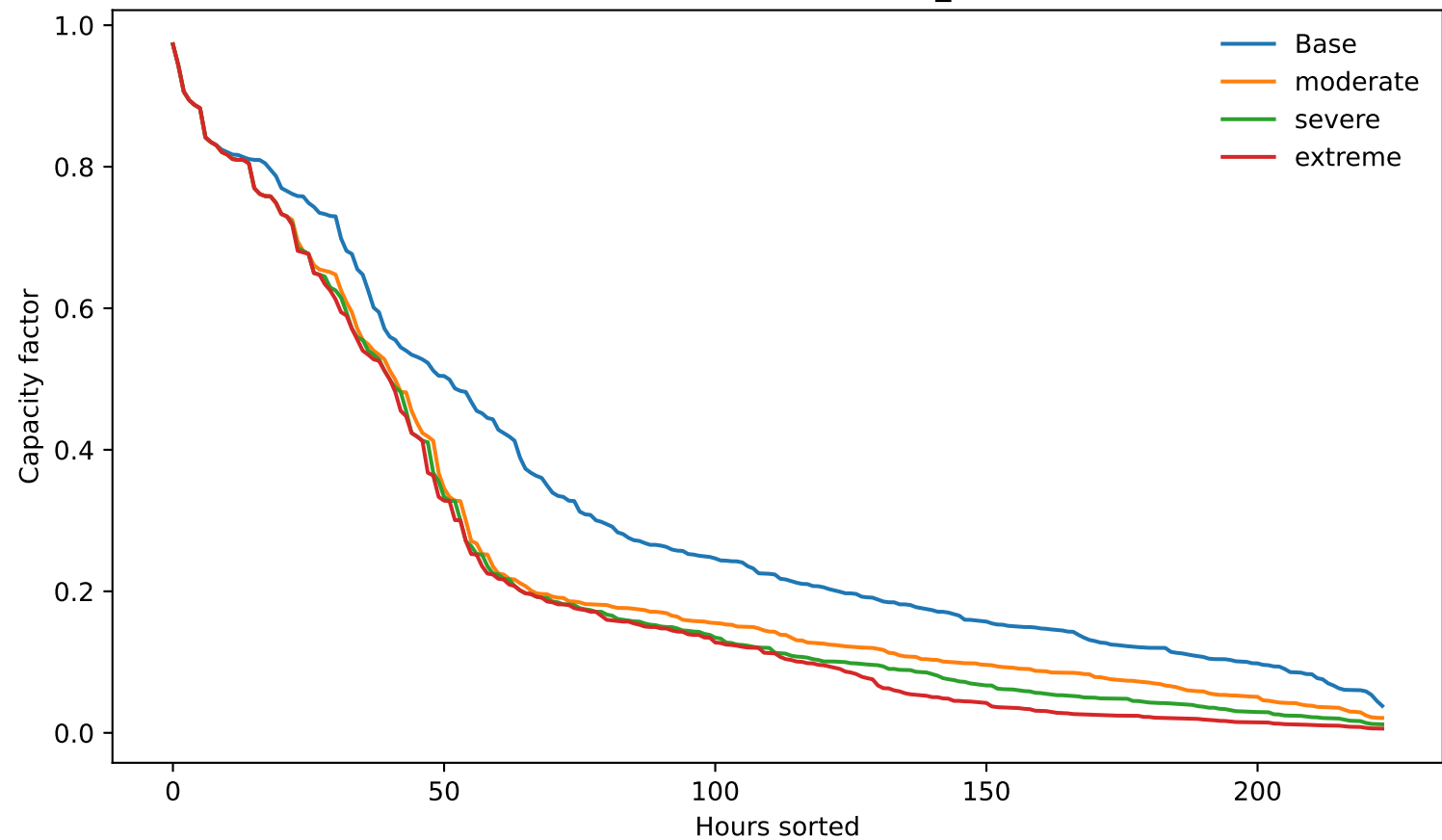
Duration curve — onshore_wind
