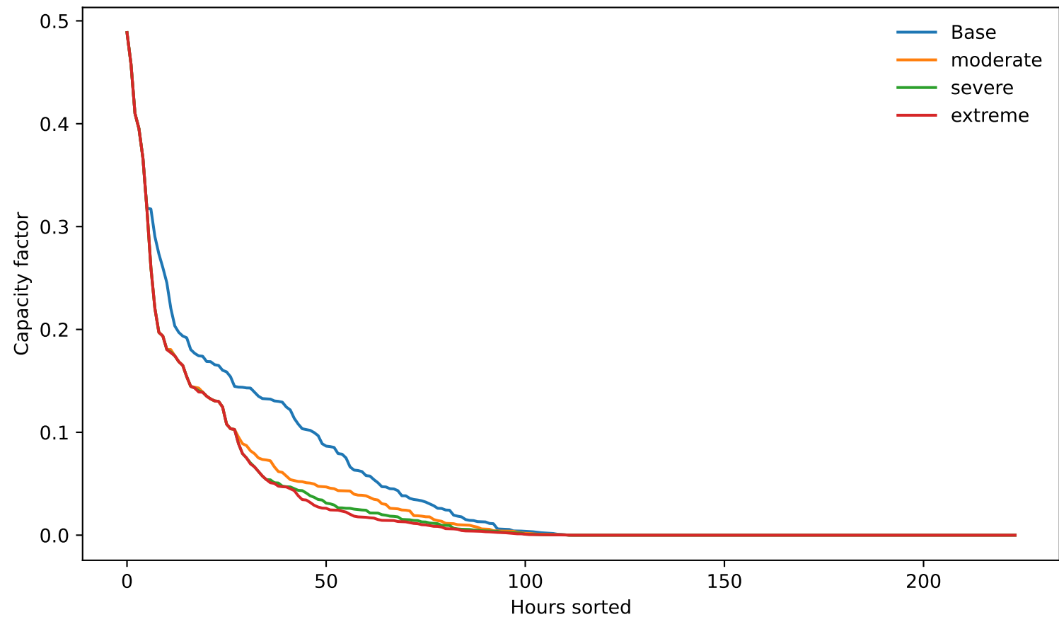
Duration curve — solar
