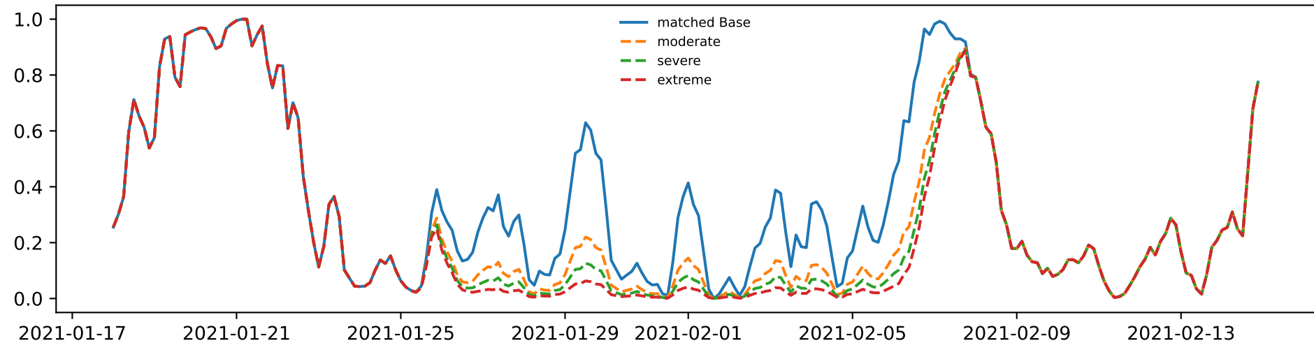
DE0 7 0 onwind
