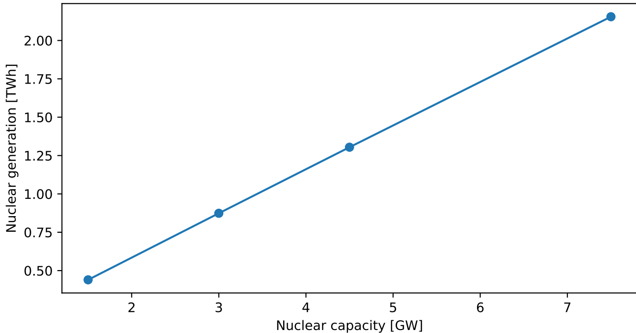
Core: nuclear capacity vs generation
