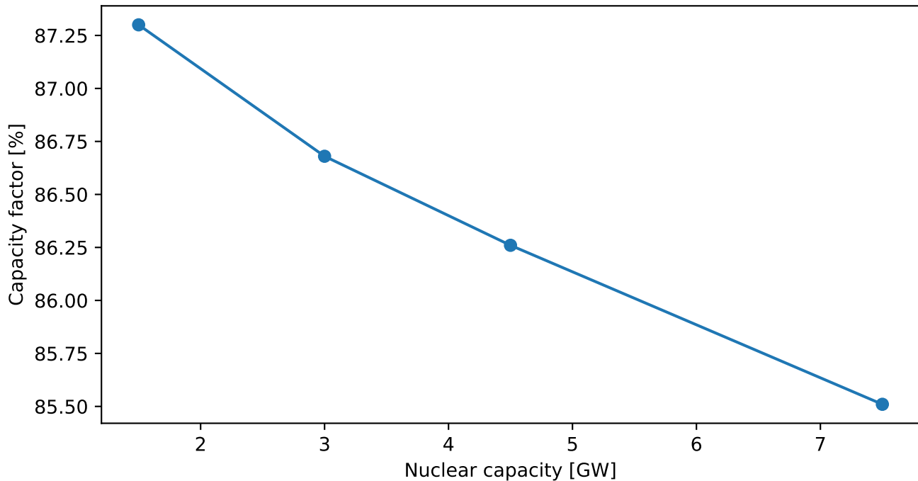
Core: nuclear capacity factor
