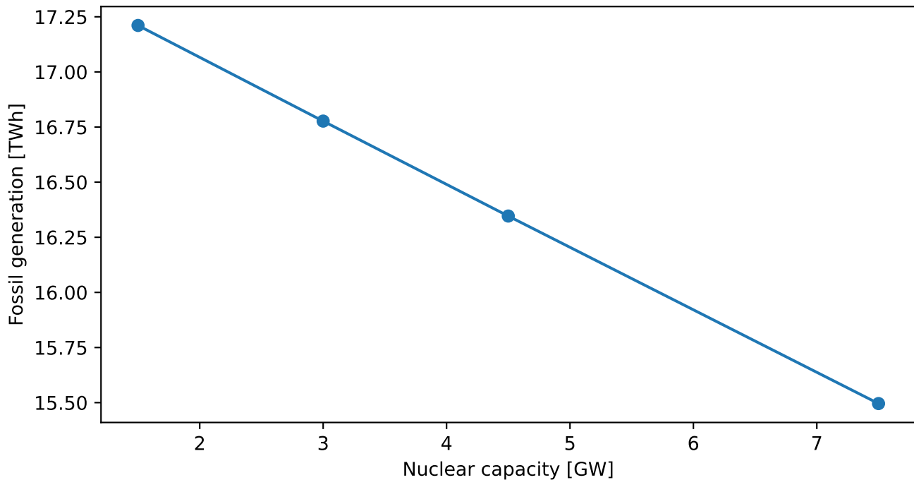
Core: fossil generation vs nuclear capacity
