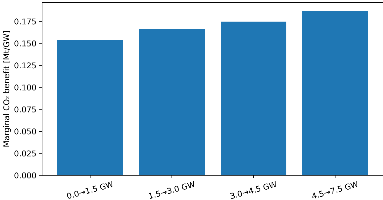
Marginal CO 2 benefit per additional GW
