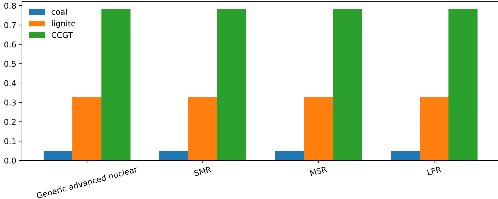
Core: fossil displacement by fuel
