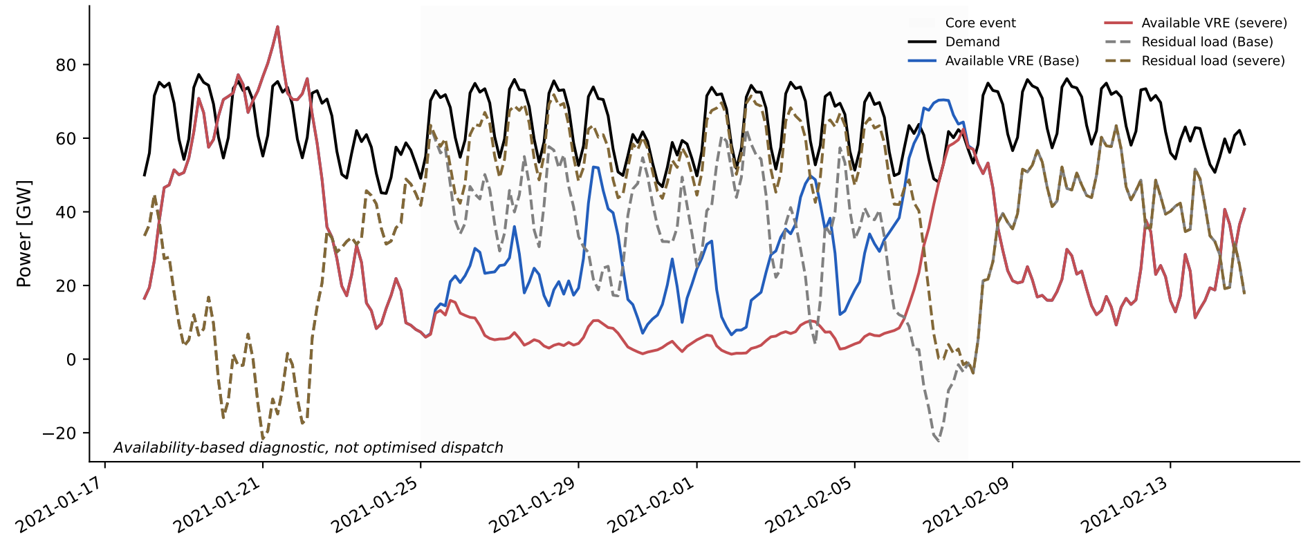
Demand, available VRE and residual load
