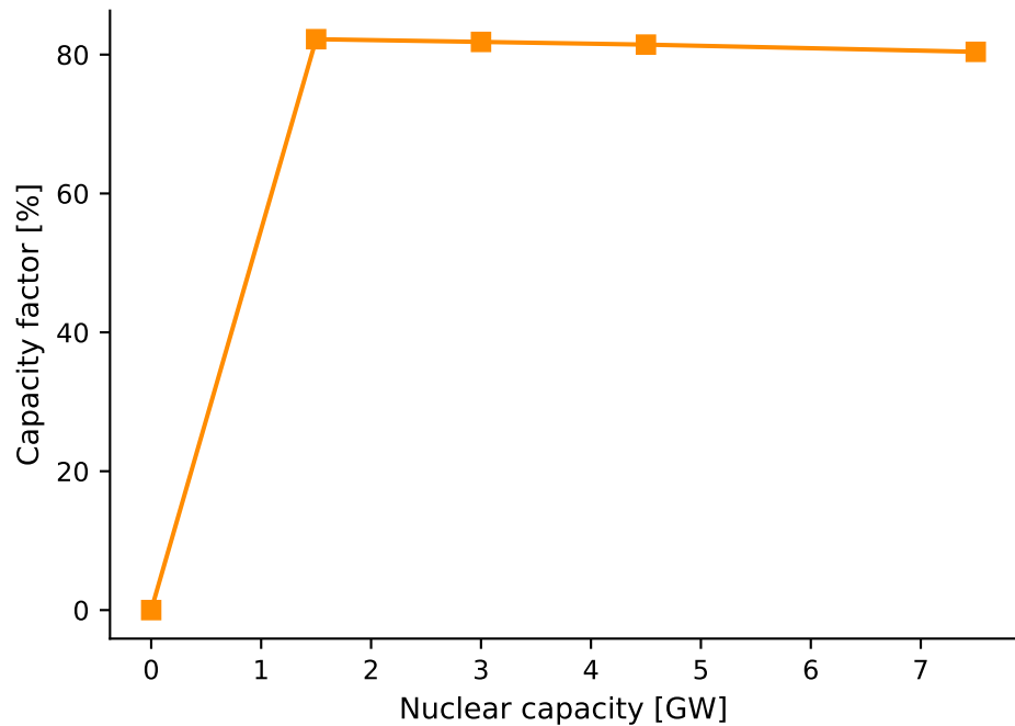
Nuclear capacity and generation
