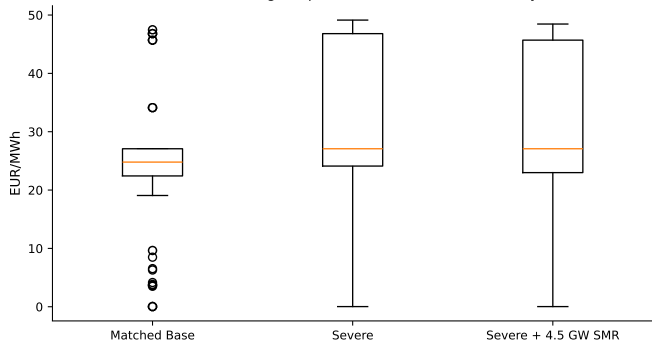
Modelled marginal-price distribution and summary
