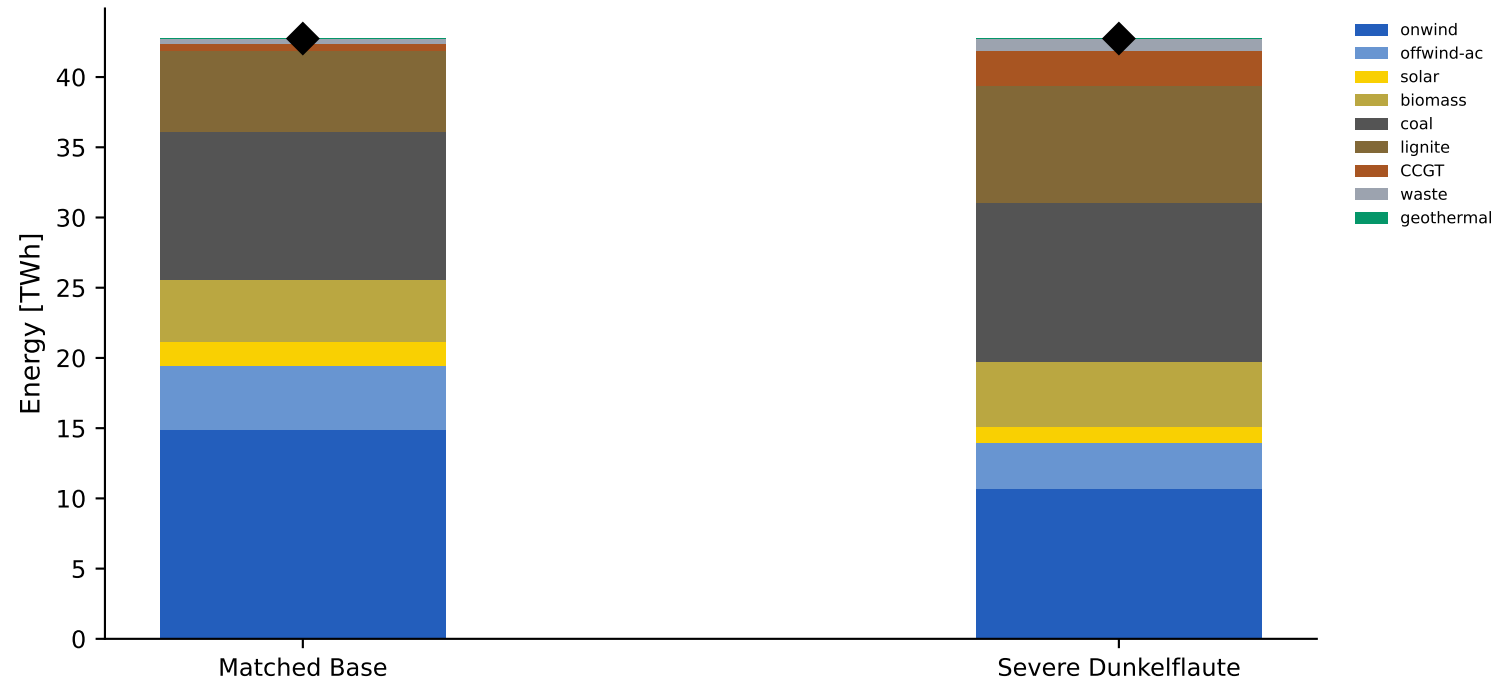
Generation mix comparison — full 28-day window
