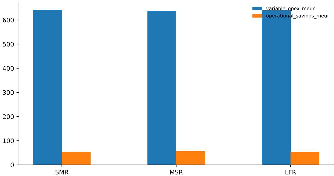
Reactor technology cost comparison (4.5 GW)
