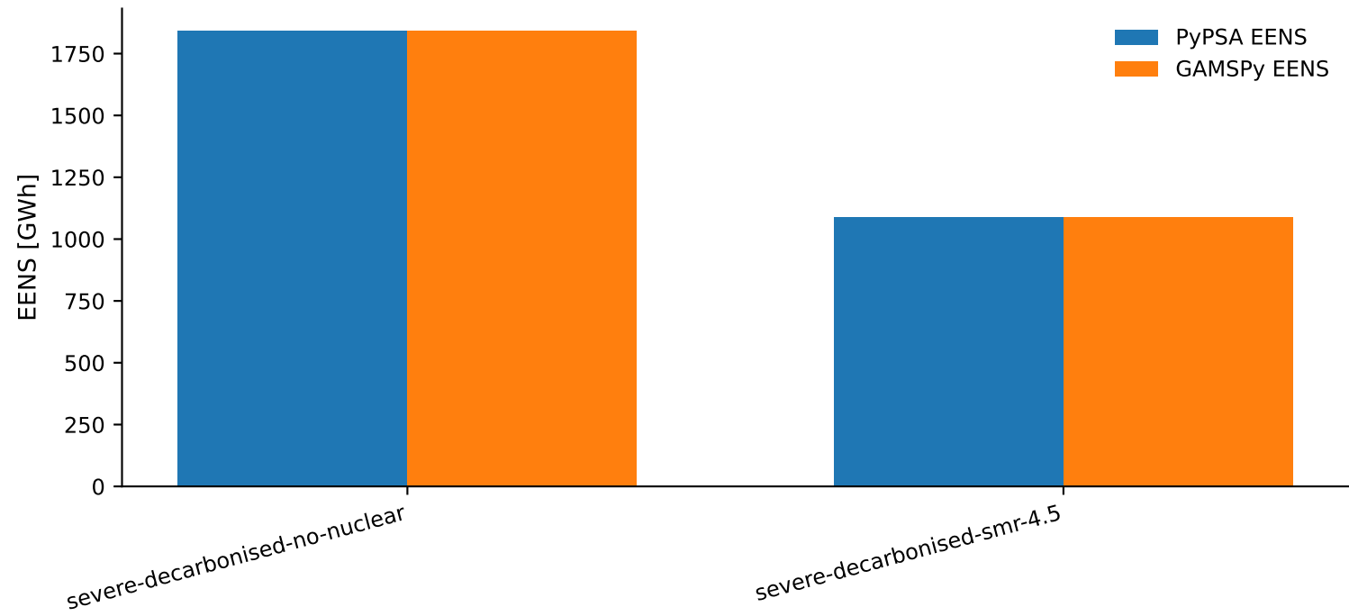
PyPSA-GAMSPy adequacy comparison
