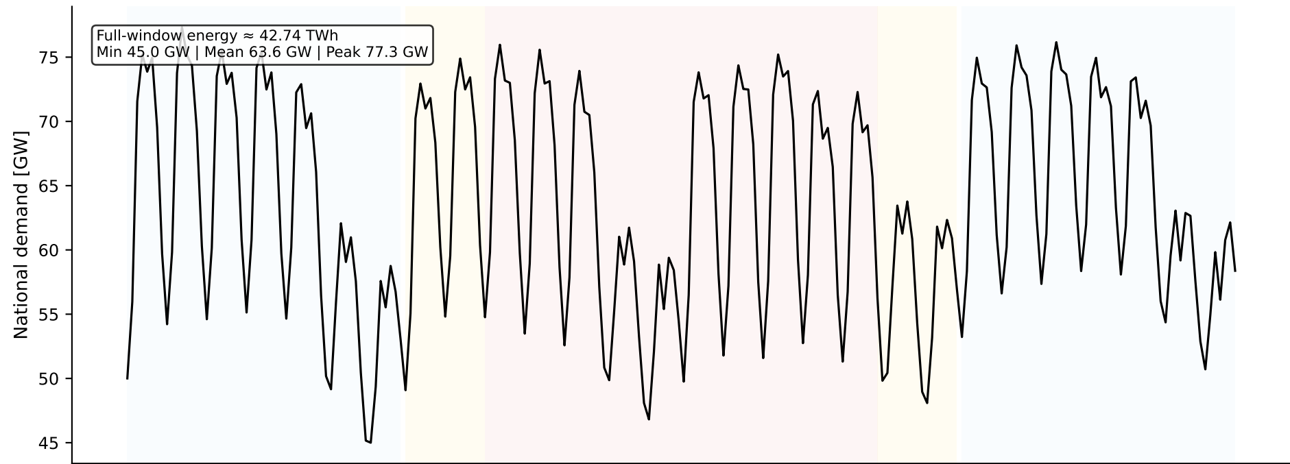
Electricity demand over the 28-day modelling window
