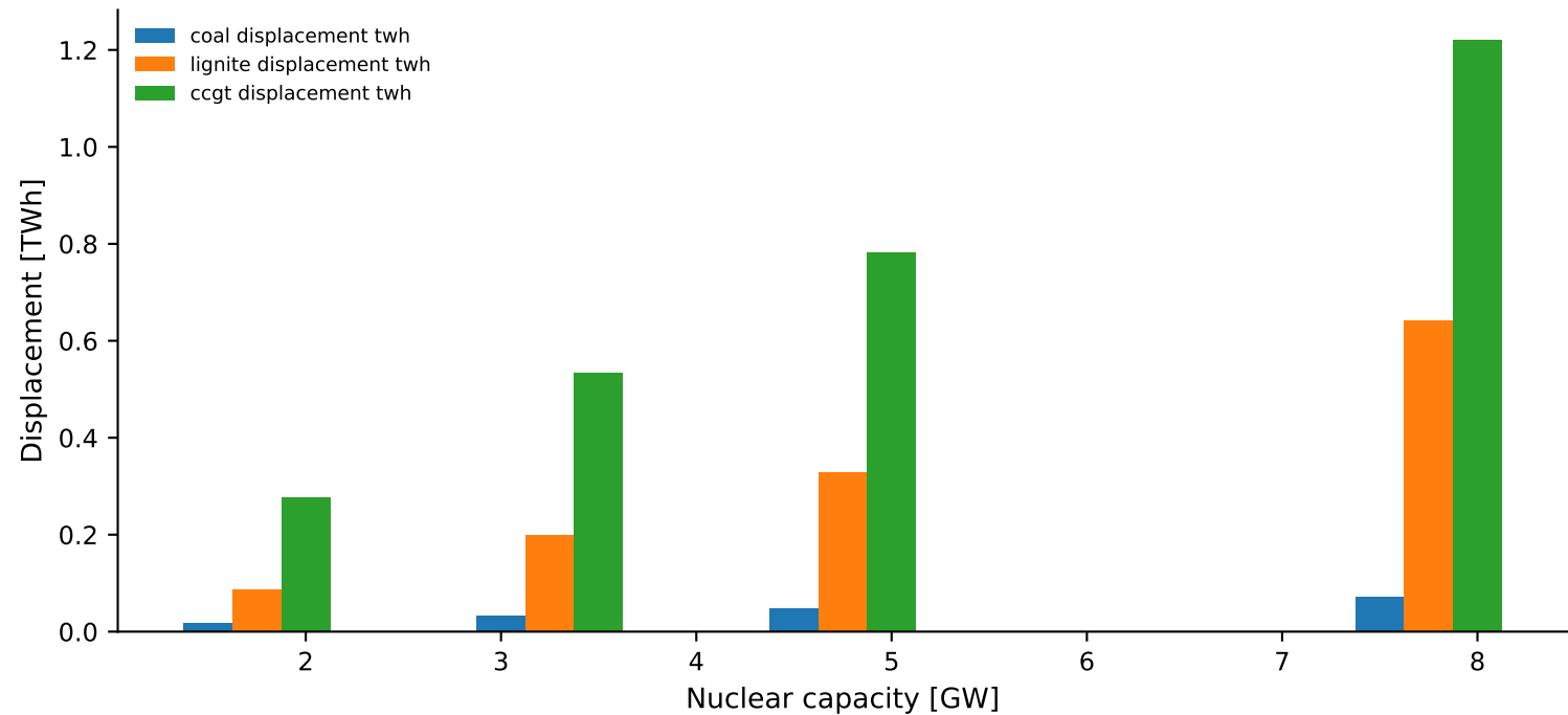
Fossil displacement by fuel
