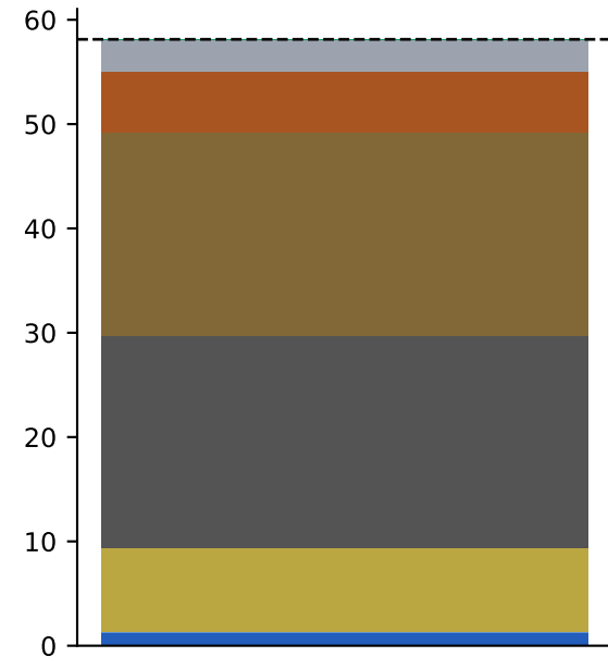
Min available VRE 2021-02-01 21:00:00
