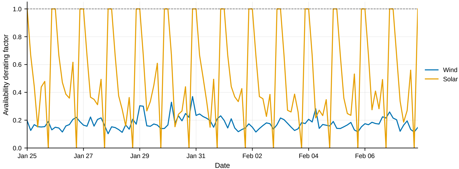
Dunkelflaute derating profile
