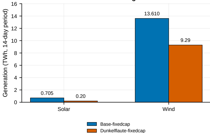
Panel A: Renewable generation
