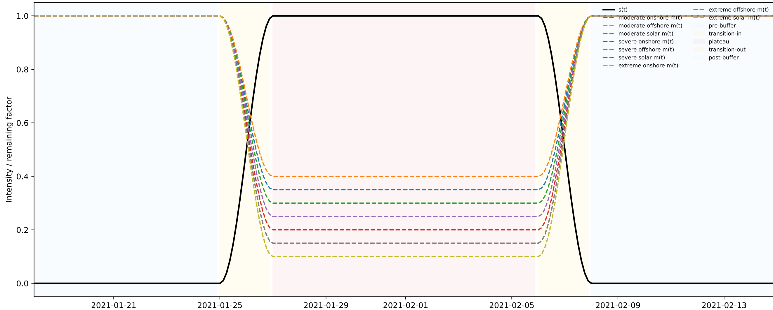
Stylised Dunkelflaute V4 stress envelope
