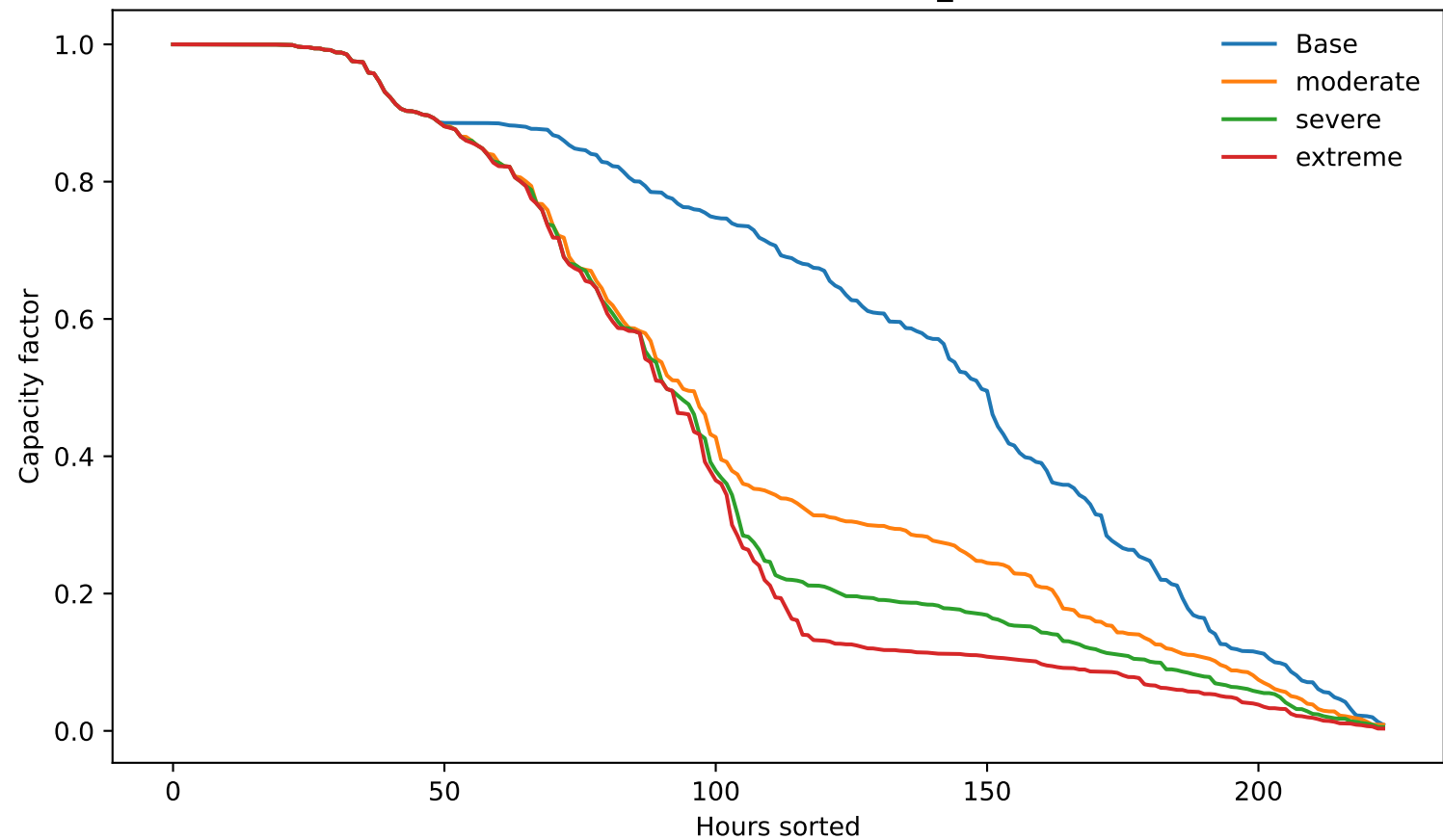
Duration curve — offshore_wind
