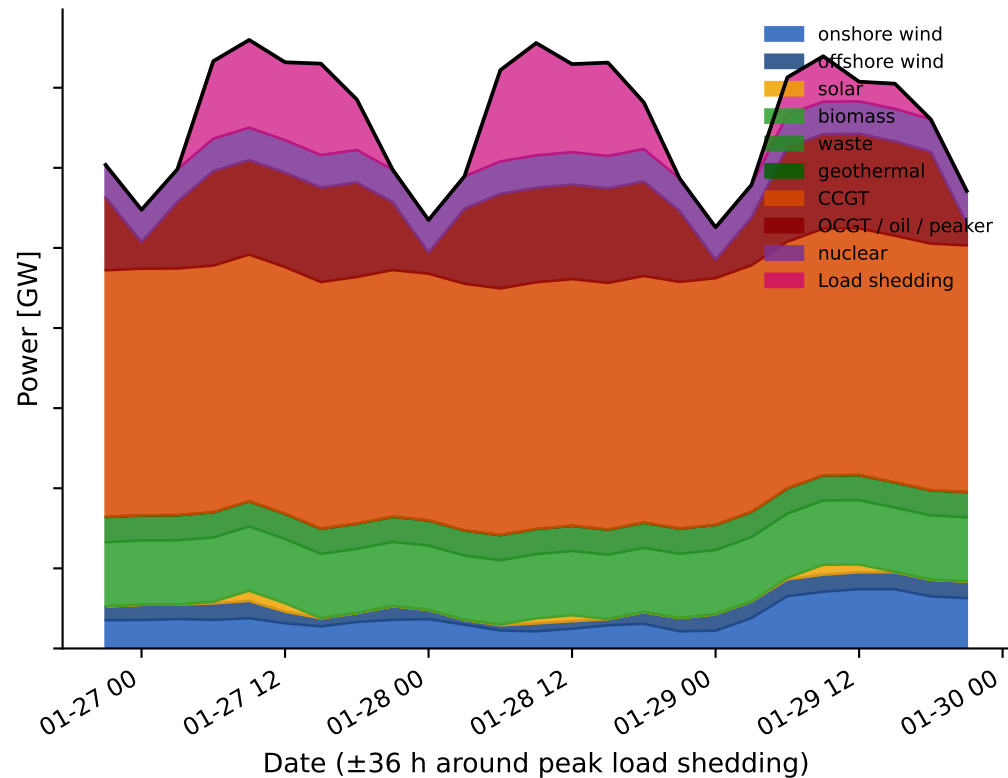
+4.5 GW SMR
