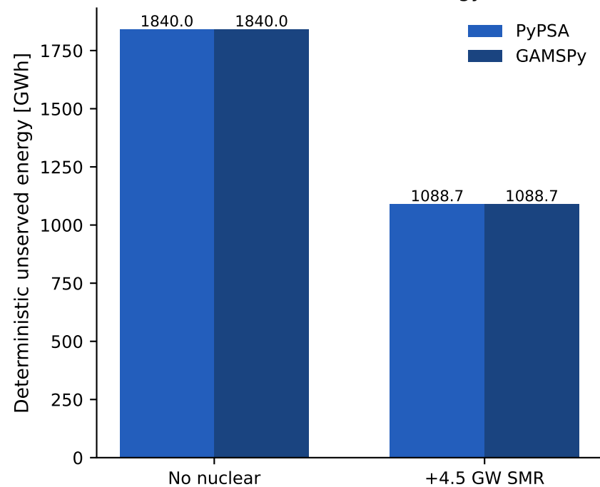
Panel A: unserved energy
