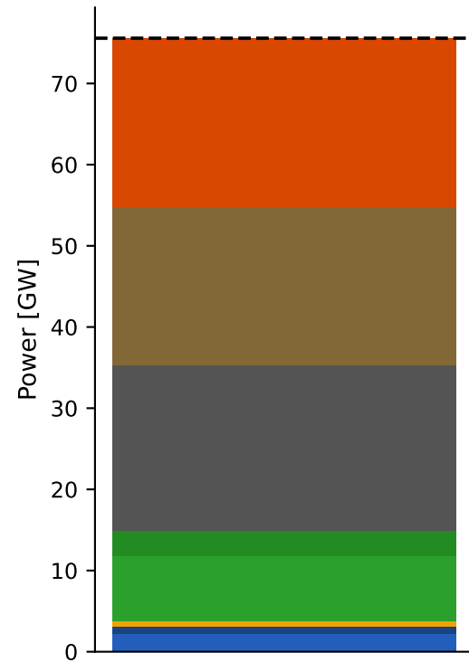
Maximum residual load 2021-01-28 09:00:00 (severe fossil-rich)
