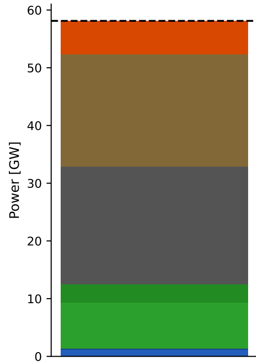
Minimum available VRE 2021-02-01 21:00:00 (severe fossil-rich)
