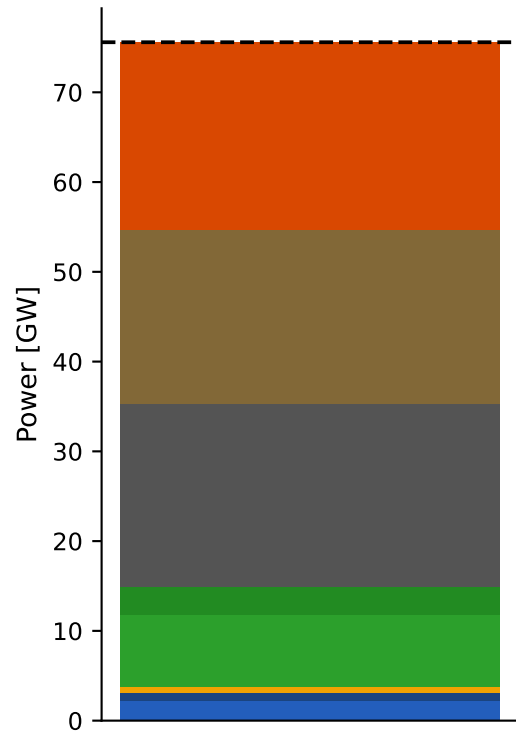
Maximum CCGT dispatch 2021-01-28 09:00:00 (severe fossil-rich)
