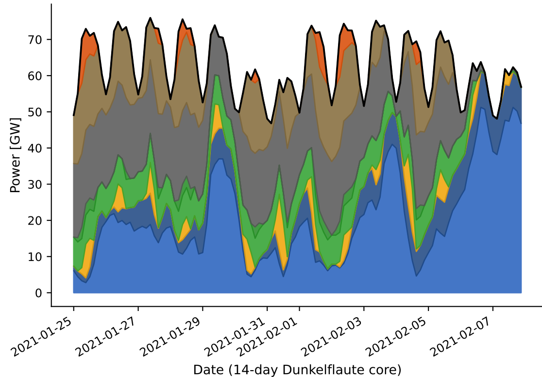
Matched reference
