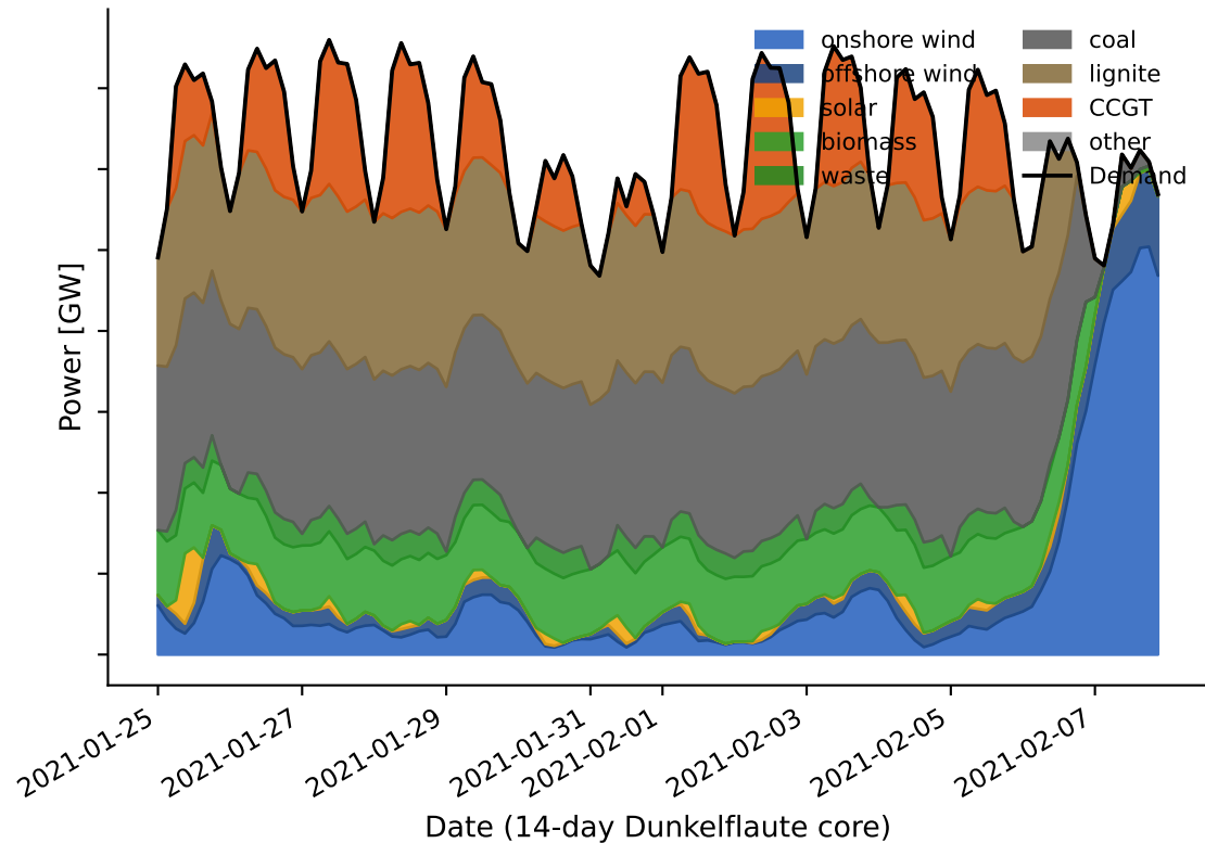
Severe
