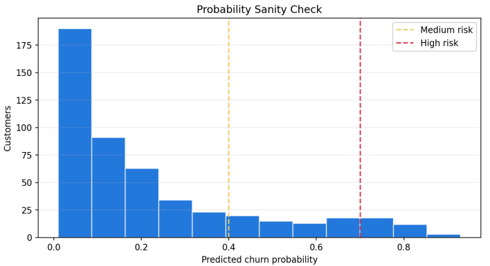
Probability distribution helps catch overconfident or collapsed scoring.
