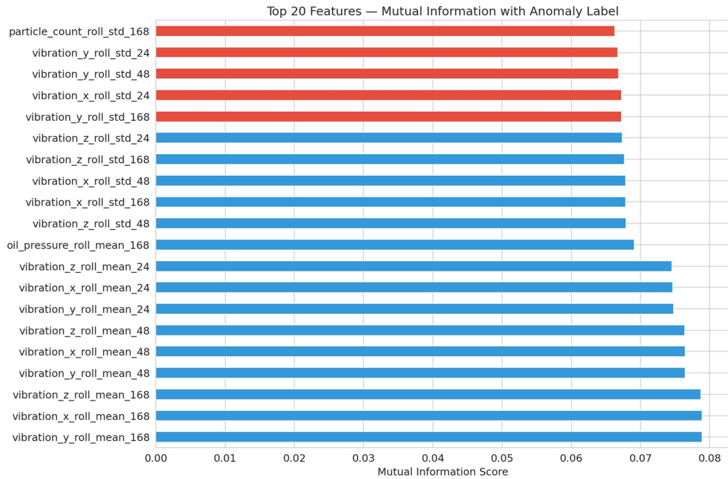
Fig. 2: Feature importance ranking by mutual information scores
