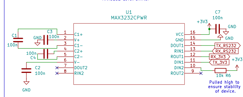
MAX3232 Level Shifter
