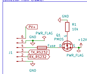
Connector from Crawler
