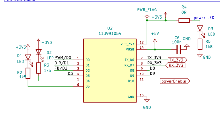
MCU with Radio
