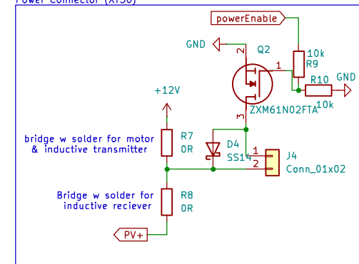
Power Connector (XT30)
