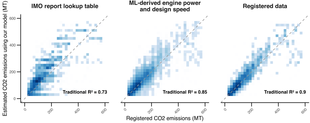
Figure 5: Comparison of daily vessel-level \text{CO}_2 emissions estimated using our model with registered emissions from a proprietary vessel database (based on main engine fuel consumption over 24 hours). Estimates are shown using main engine power and design speed from IMO (left), our machine learning random forest models (center), and the same registered dataset (right). The dashed line represents the 1:1 line. Performance values for traditional R^2 are shown for each set of vessel characteristics. Over 16,000 vessels are represented in the figure, and blue shading indicates point density. All data are rule-of-three compliant, meaning each cell (20x20 mt) displayed contains at least three vessels.
