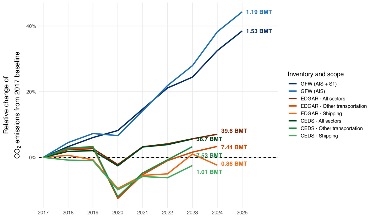
Figure 27: Marine emissions growth against all sectors and against other transport modes, in EDGAR and CEDS, indexed to 2017.
