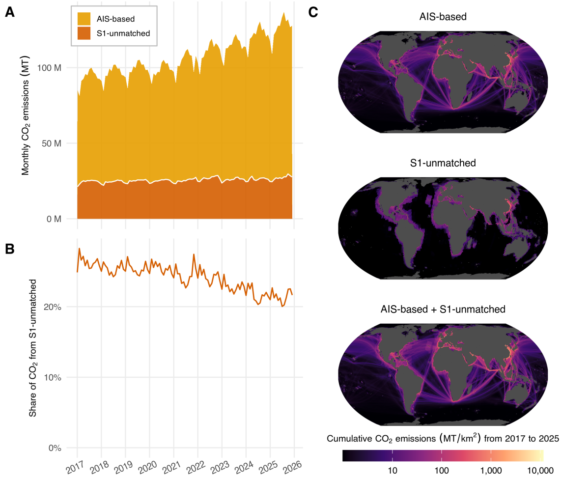
Figure 2: (A) Time series of monthly global CO 2 emissions, shown for both AIS-based and S1-unmatched emissions. (B) Time series of the monthly share of global CO 2 emissions that is S1-unmatched. (C) Spatial distribution of cumulative 2017-2025 CO 2 emissions, AIS-based (top), S1-unmatched (middle), and combined (bottom), shown at a 1x1 degree spatial resolution; emissions are area-normalized for each pixel (metric tonnes per square kilometer, shown on a pseudolog-10 scale).
