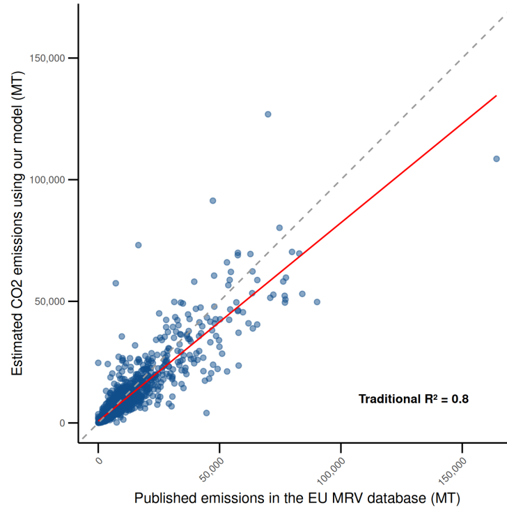
Figure 6: Comparison of annual vessel-level CO 2 emissions estimated using our model with published emissions from the EU MRV database. The sample includes 2,276 observations from yearly aggregated vessel trips where hours at sea differ by no more than 15% between our data and the MRV dataset. The solid red line shows the linear regression fit, and the dashed line represents the 1:1 line.
