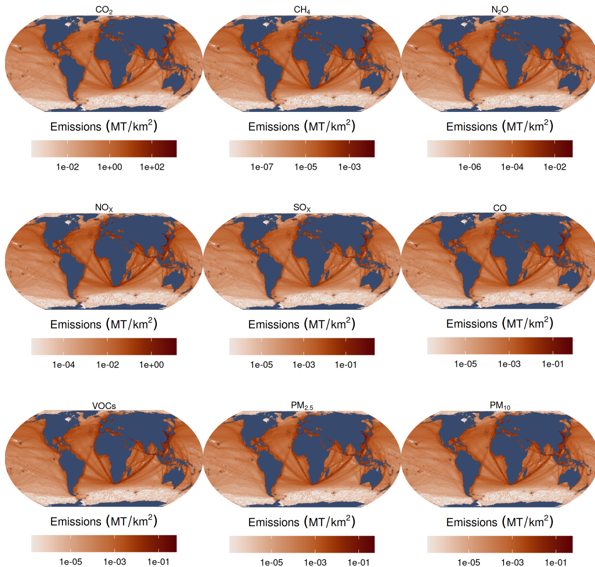
Figure 17: Spatial maps 2024 emissions for each GHG and pollutant, aggregated across AIS-broadcasting vessels and non-broadcasting vessels, and shown at a 1x1 degree spatial resolution. Emissions are area-normalized for each pixel (metric tonnes per square kilometer), and shown using a log-10 scale.
