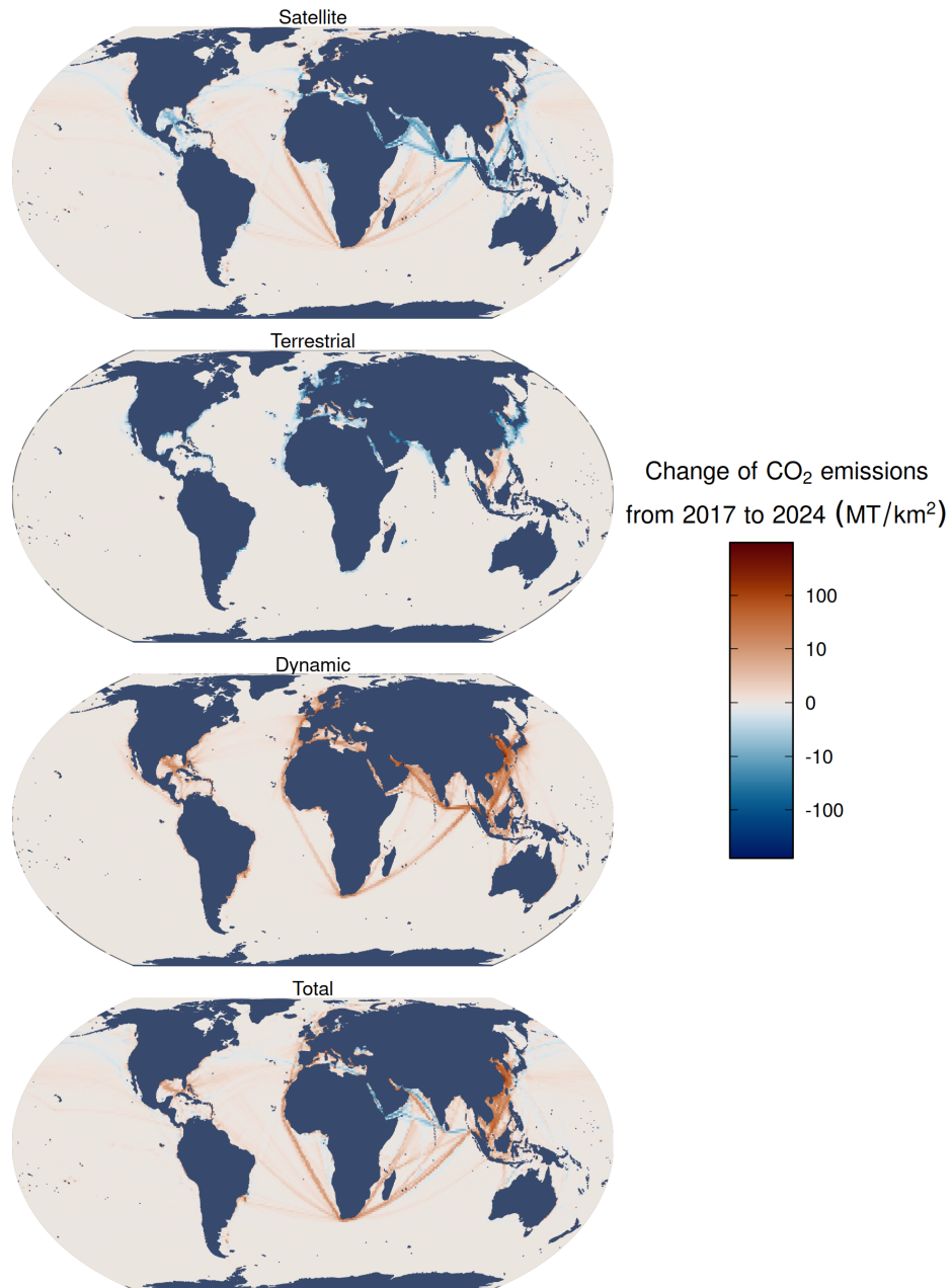
Figure 23: Spatial change in CO 2 emissions by AIS-broadcasting vessels between 2017 and 2024 (metric tonnes) by receiver type (satellite, terrestrial, and dynamic) and total across receiver types, at a 1x1 degree spatial resolution; emissions are area-normalized for each pixel (metric tonnes per square kilometer, shown on a pseudolog-10 scale).
