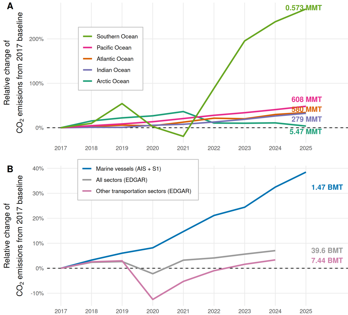
Figure 4: (A) Trend in CO 2 emissions by ocean (normalized to 2017 baseline), use our fused AIS+S1 marine vessel data. (B) Comparison in trend of CO 2 emissions data (normalized to 2017 baseline) between marine transportation emissions from GFW, other transportation emissions from EDGAR, and all sector emissions from EDGAR. On the right-hand side of the figure, 2024 absolute values (in millions of metric tonnes) are shown as text and color-coded for each line.
