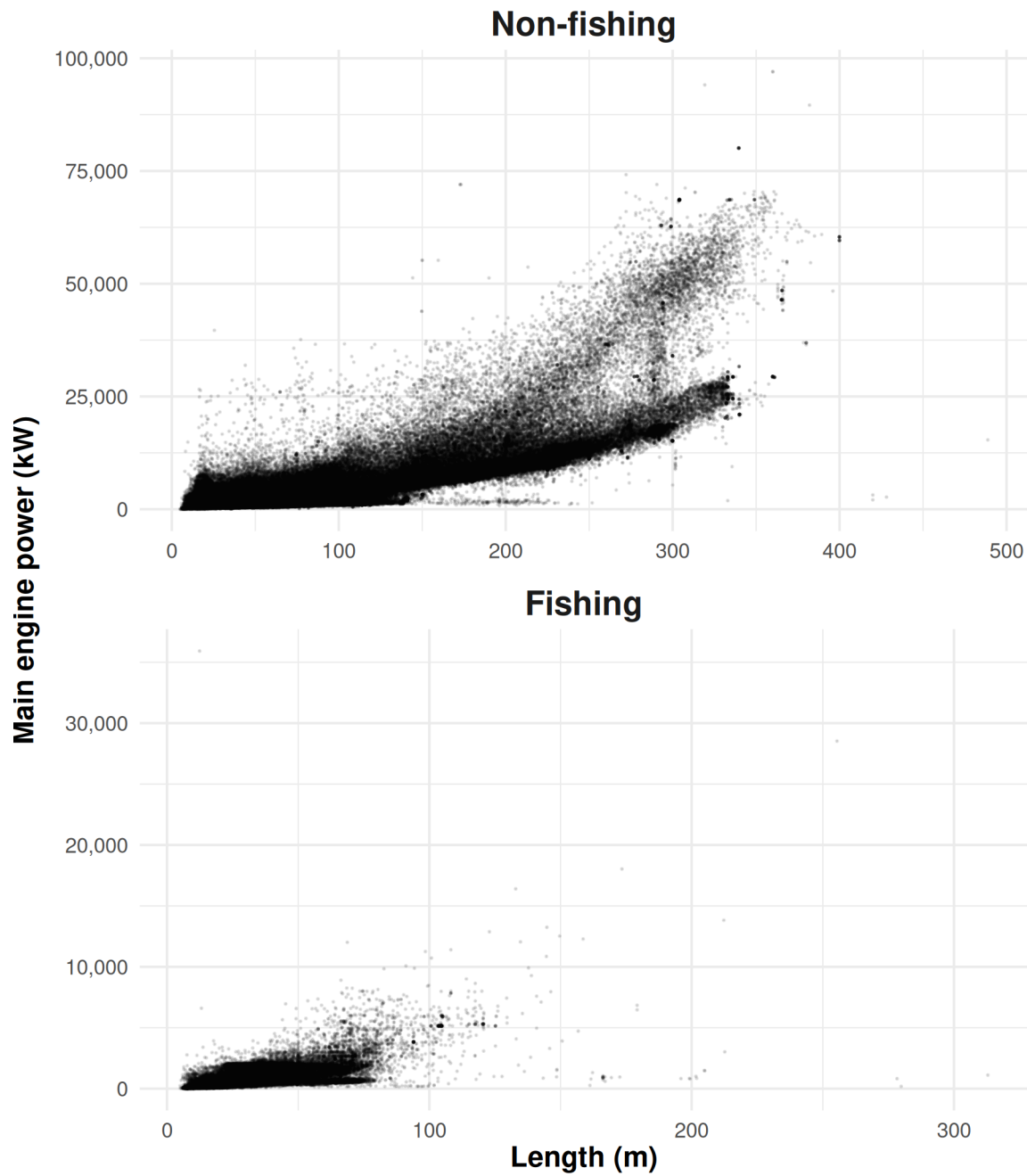
Figure 9: Relationship between main engine power (killowatts) and length (meters) for all AIS-broadcasting vessels, disaggregated by non-fishing and fishing vessels.
