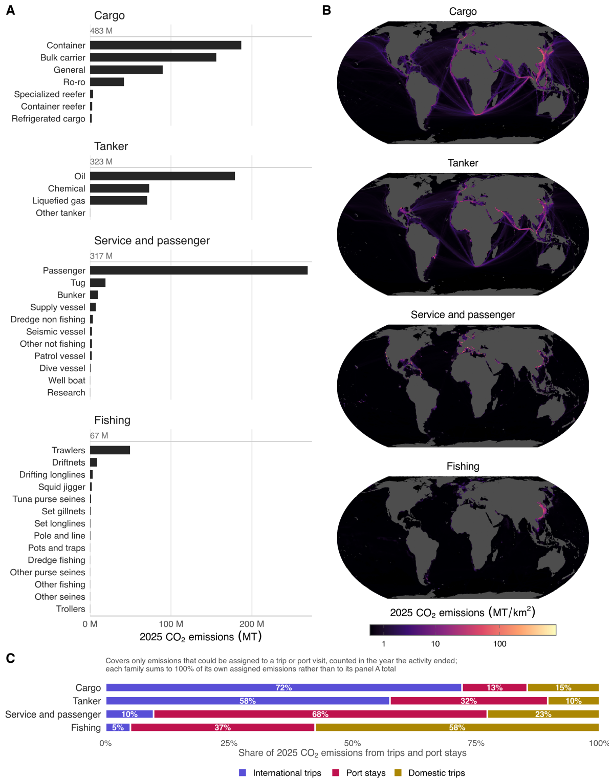
Figure 3: Richness of AIS-broadcasting vessel emissions data, showing: (A) Total 2025 CO 2 emissions by vessel class for AIS-broadcasting vessels. Vessel classes are grouped into four families, with the total for each family shown above its bars; every class in a family is shown as its own bar, so panel heights differ with the number of classes. These totals are aggregated from the same gridded emissions shown in panel B, so the two panels describe exactly the same emissions and the bars sum to the mapped total. (B) Spatial distribution of 2025 CO 2 emissions from AIS-broadcasting vessels for each of those same vessel class families, shown at a 1x1 degree spatial resolution;
