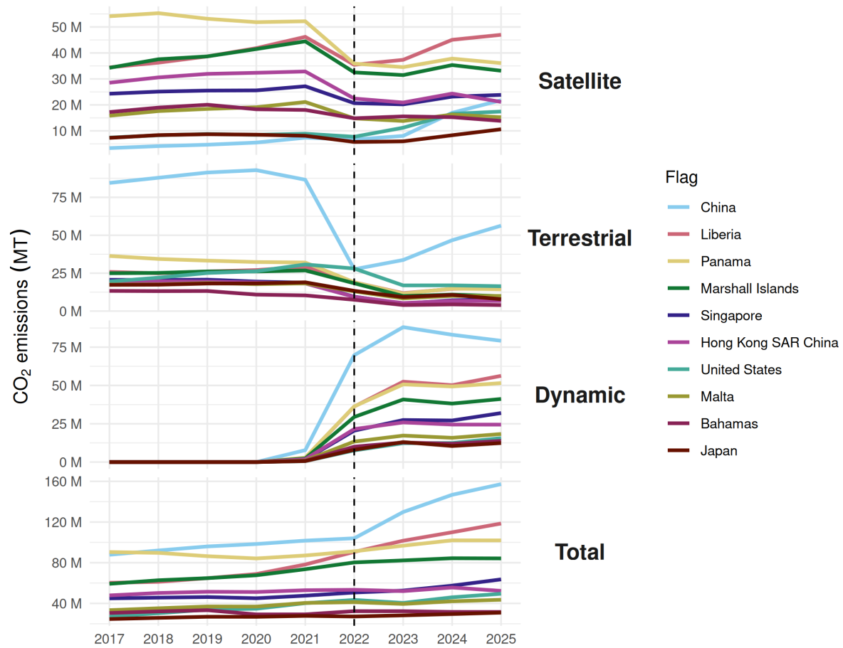
Figure 22: Annual total CO 2 emissions (metric tonnes) by AIS-broadcasting vessels, disaggregated by AIS receiver type (satellite, terrestrial, and dynamic) and total aggregated across receiver types, for the top 10 flags with the most emissions in 2025. A dashed vertical line is shown for 2022, the first year in which dynamic AIS was widely adopted.
