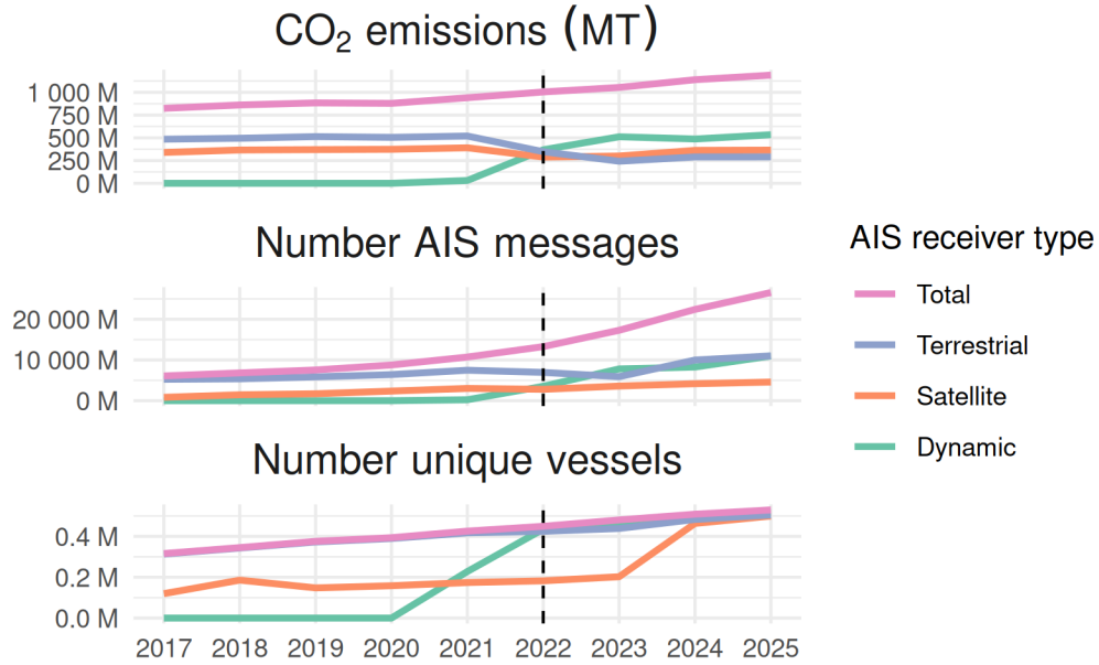
Figure 21: Annual total CO 2 emissions (metric tonnes) by AIS-broadcasting vessels, AIS pings (i.e., individual vessel timestamped location messages), and number of unique AIS-broadcasting vessels. Trends are disaggregated by AIS receiver type (satellite, terrestrial, and dynamic), and also shown as a total aggregated across receiver types. A dashed vertical line is shown for 2022, the first year in which dynamic AIS was widely adopted.
