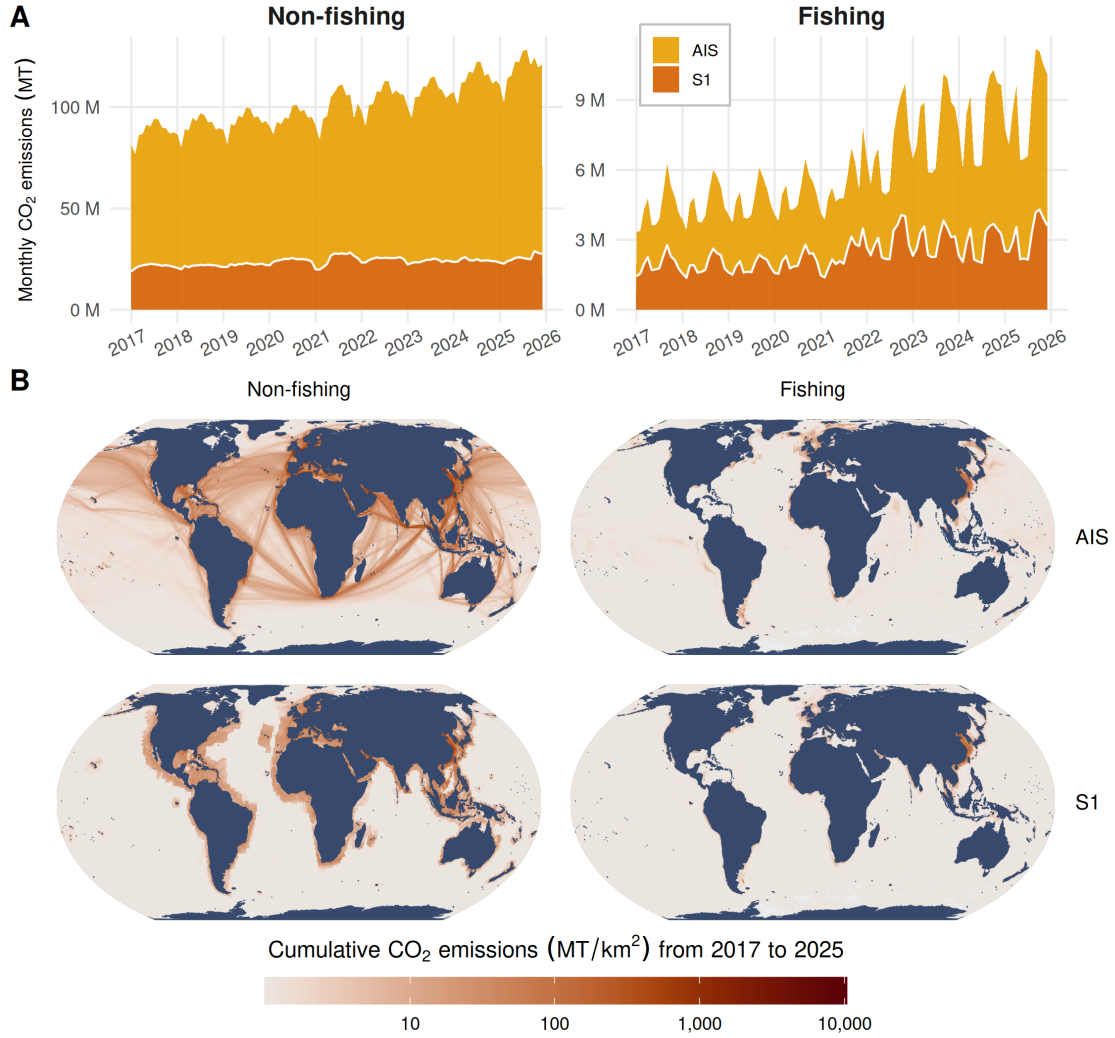
Figure 2: (A) Time series of monthly global CO 2 emissions, shown for both AIS-broadcasting and S1-detected non-broadcasting vessels, and for both fishing and non-fishing vessels. (B) Spatial distribution of cumulative 2017-2025 CO 2 emissions from both AIS-broadcasting and S1-detected non-broadcasting vessels, for both fishing and non-fishing vessels, and shown at a 1x1 degree spatial resolution; emissions are area-normalized for each pixel (metric tonnes per square kilometer, shown on a pseudolog-10 scale).
