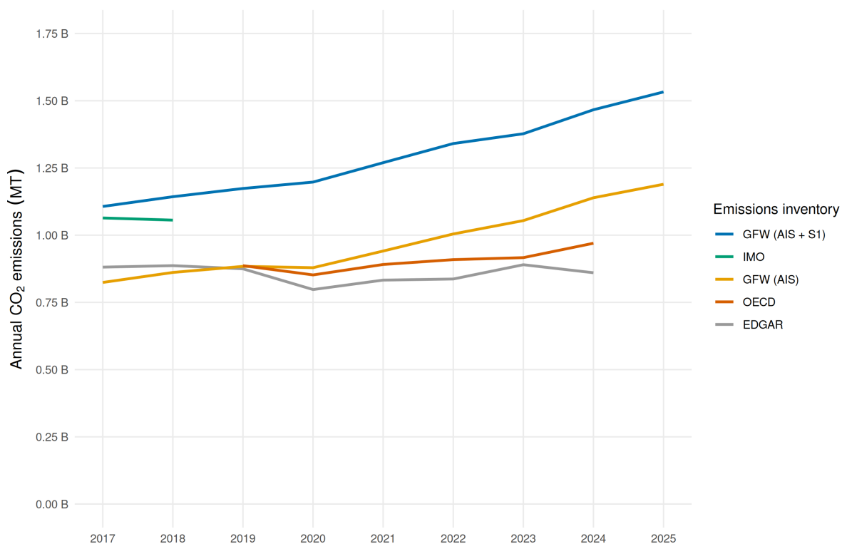
Figure 20: Comparison of annual marine vessel CO 2 emissions inventory estimates.
