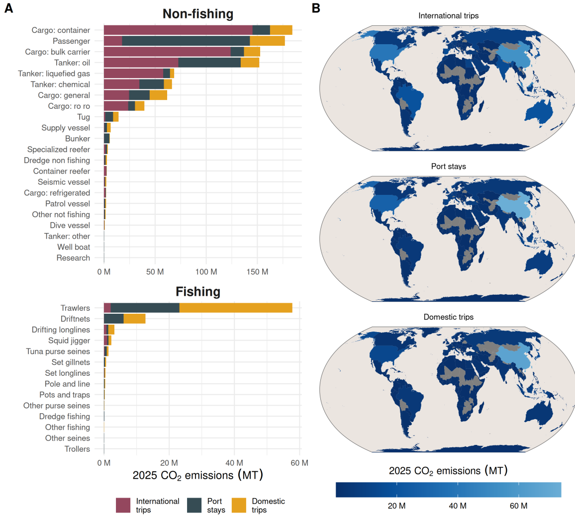
Figure 3: Richness of AIS-broadcasting vessel emissions data, showing: (A) CO 2 emissions by vessel type for AIS-broadcasting vessels during different activity types (international trips, port stays, and domestic trips), aggregated for activities ending in 2025. (B) CO 2 emissions by country for AIS-broadcasting vessels during different activity types (international trips, port stays, and domestic trips), aggregated for activities ending in 2025. For both panels, emissions for each international trip are partitioned equally to its departure and arrival country). Countries with no values are shown in black.
