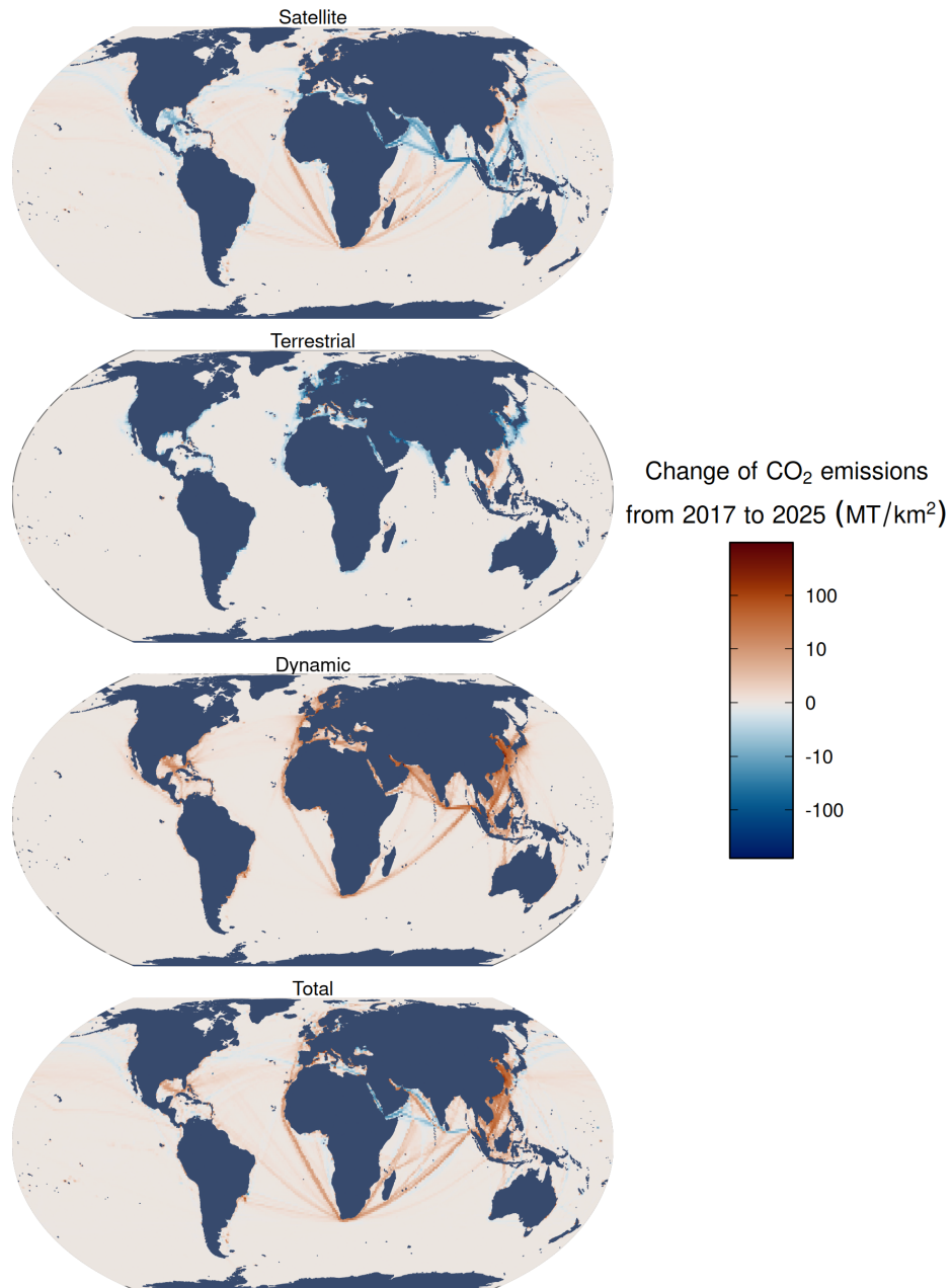
Figure 23: Spatial change in CO 2 emissions by AIS-broadcasting vessels between 2017 and 2025 (metric tonnes) by receiver type (satellite, terrestrial, and dynamic) and total across receiver types, at a 1x1 degree spatial resolution; emissions are area-normalized for each pixel (metric tonnes per square kilometer, shown on a pseudolog-10 scale).
