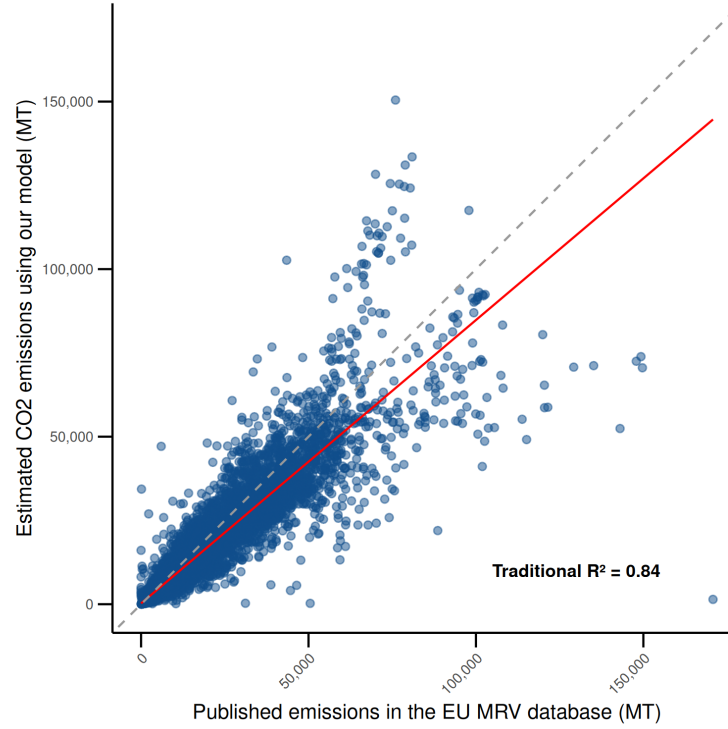
Figure 6: Comparison of annual vessel-level CO 2 emissions estimated using our model with published emissions from the EU MRV database. The sample includes 20,432 observations from yearly aggregated vessel trips where hours at sea differ by no more than 10% between our data and the MRV dataset. The solid red line shows the linear regression fit, and the dashed line represents the 1:1 line.
