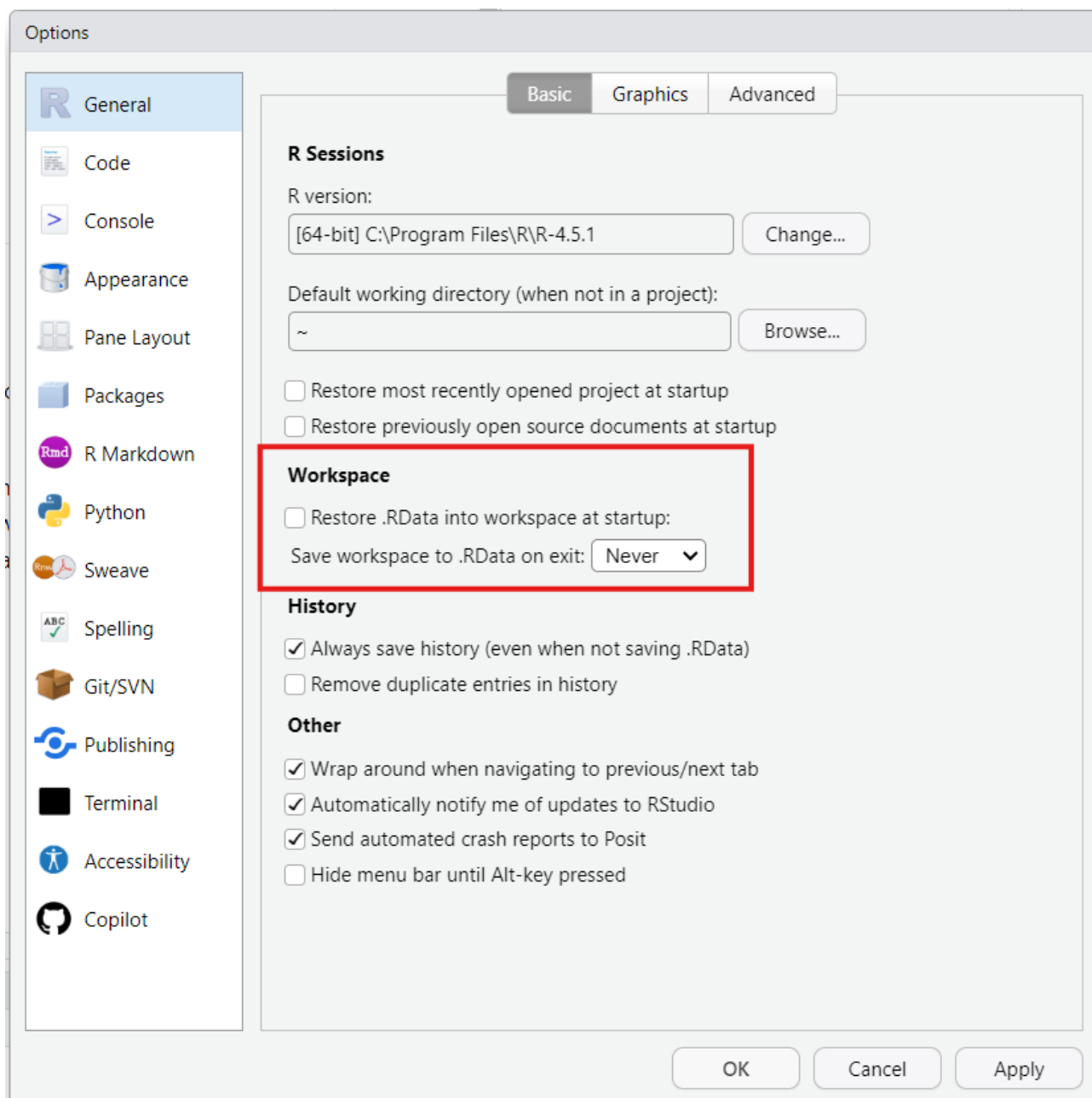
Figure 1: Global options window with recommended General settings
