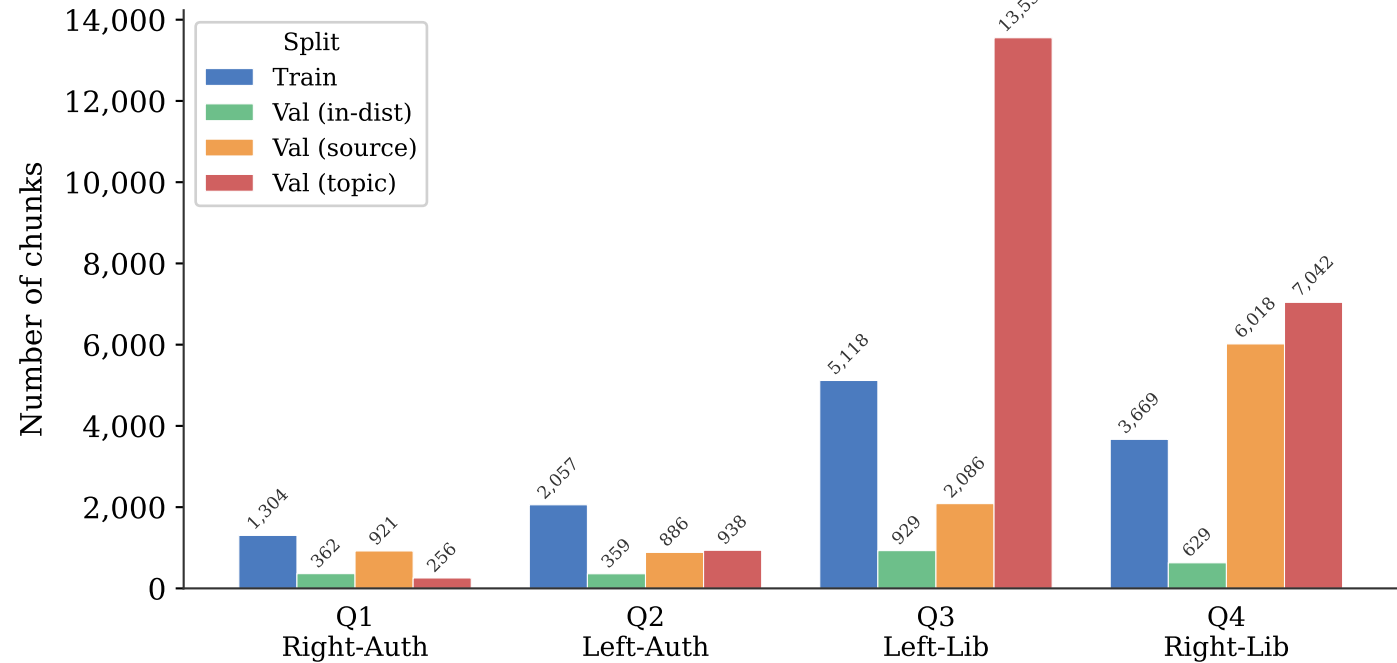
Dataset split sizes per expert
