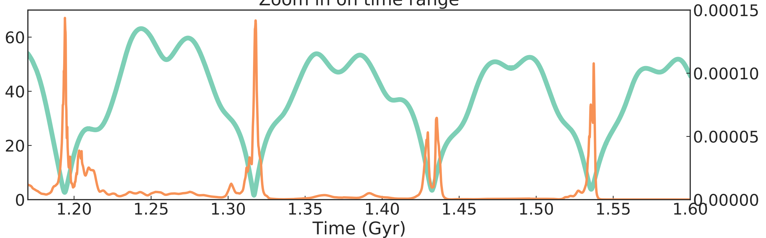
Zoom in on time range
