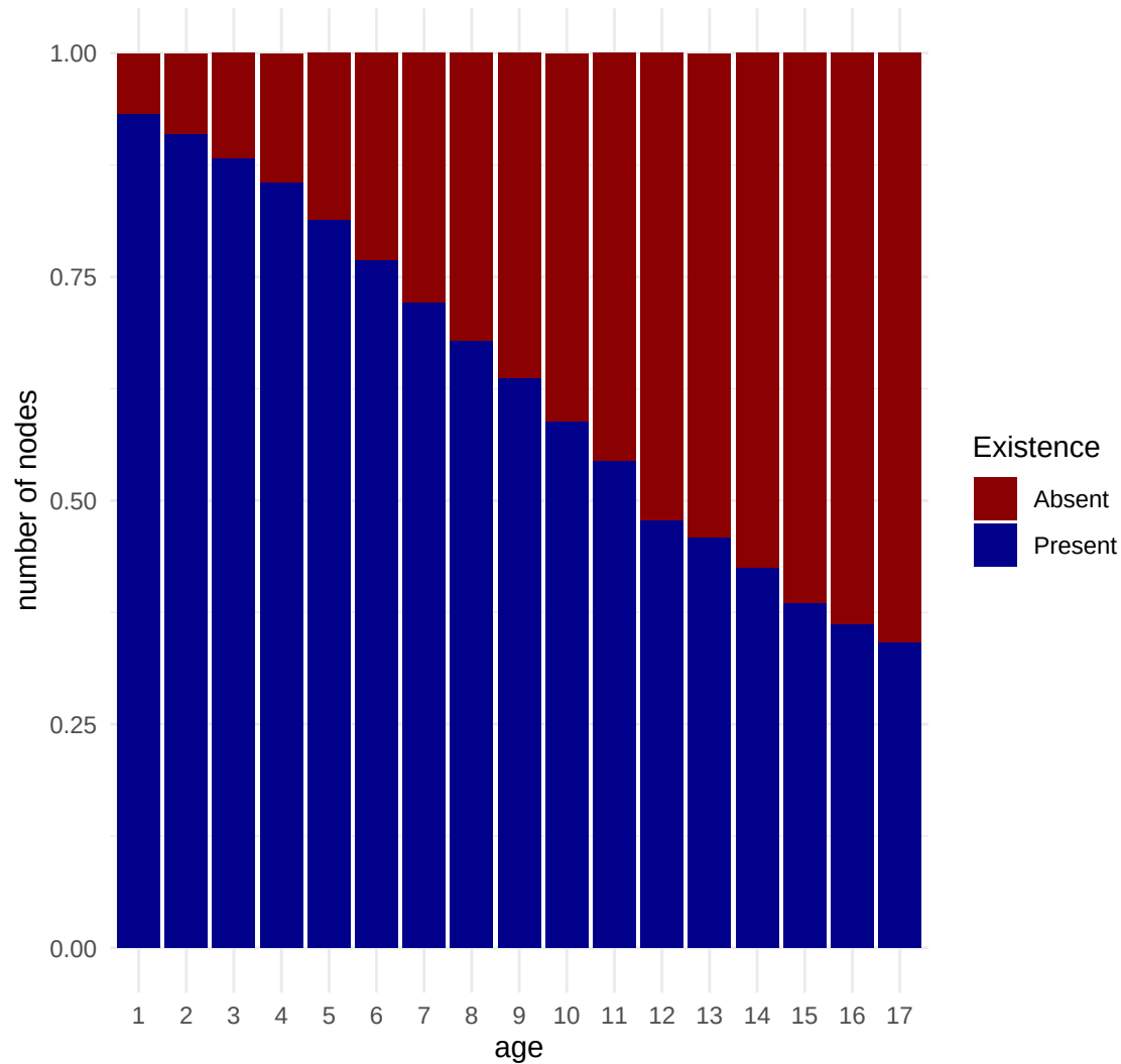
MCC
