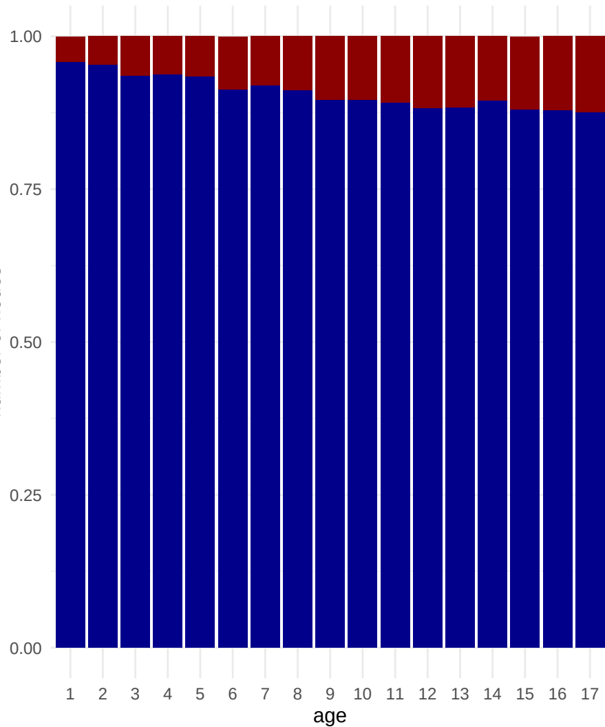
Consensus
