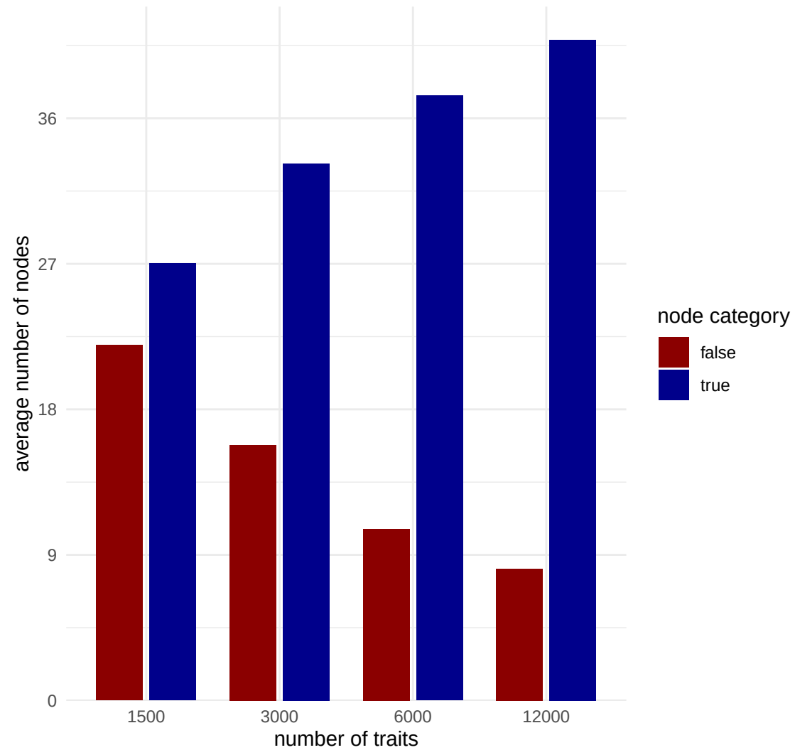
MCC
