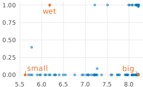
Indo-European
