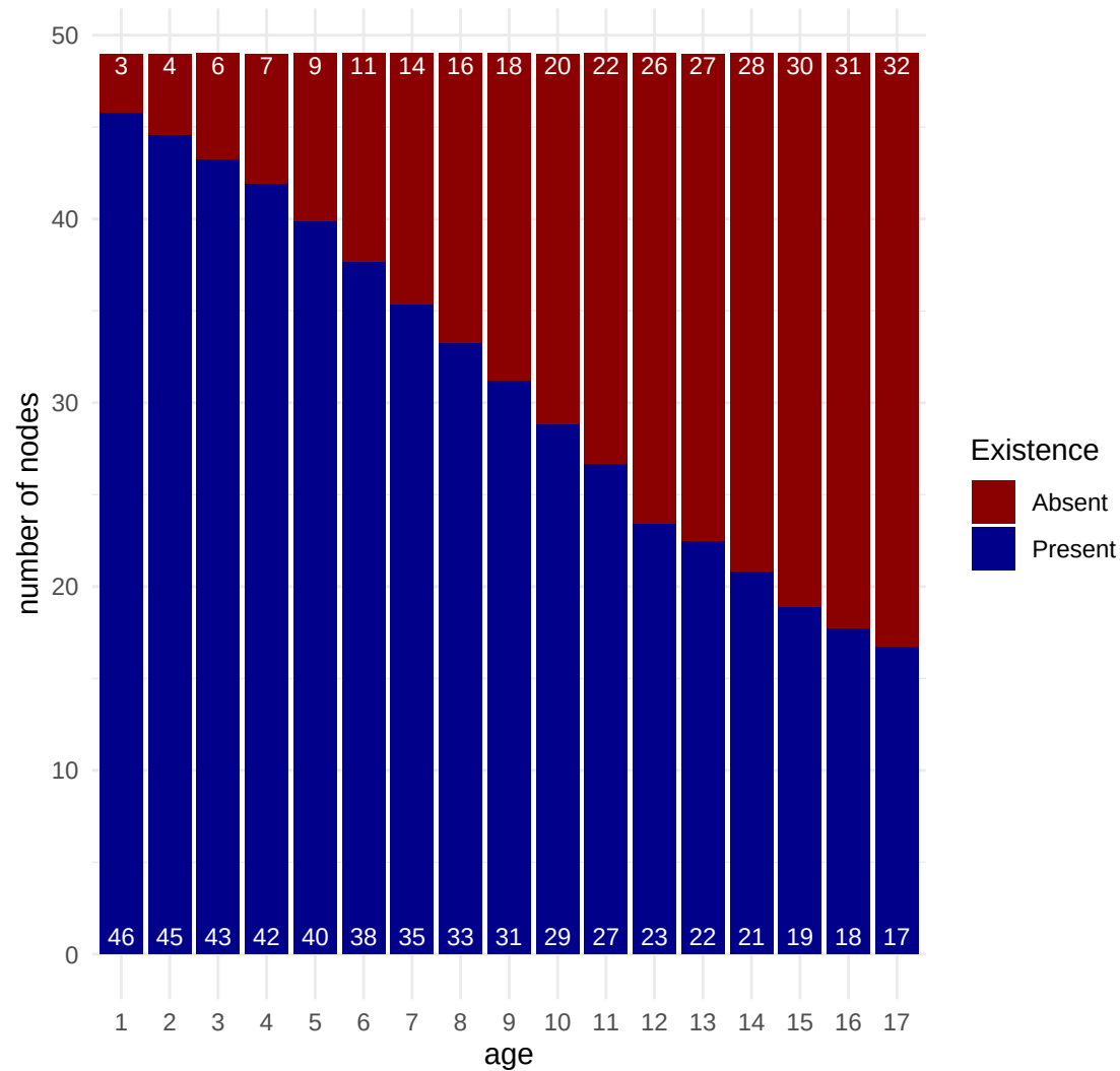
MCC
