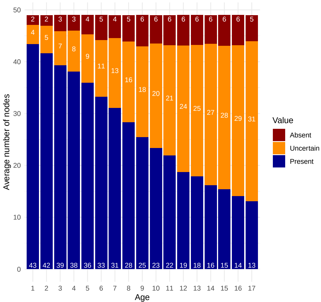
Consensus
