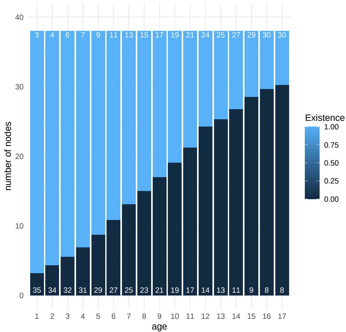
MCC
