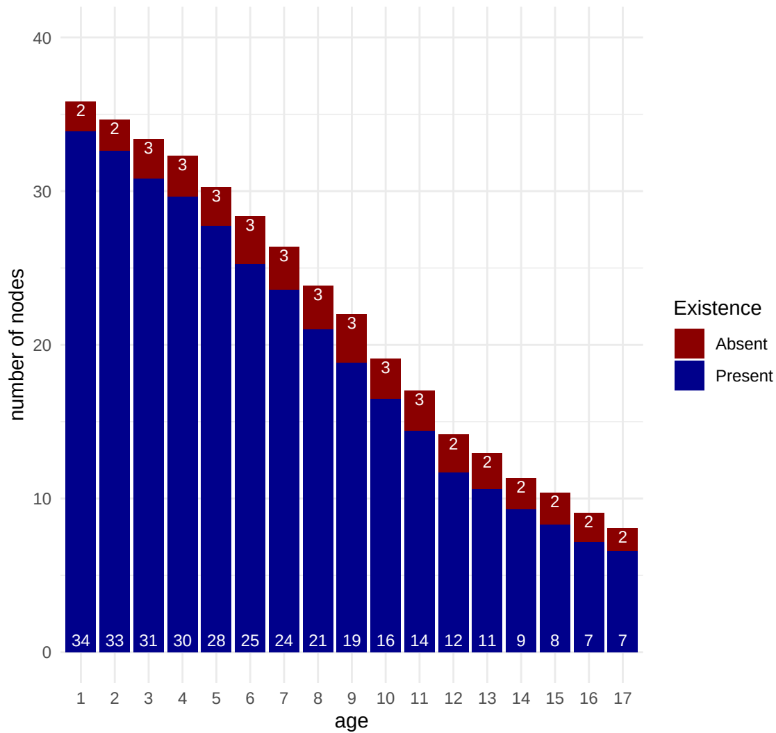
Consensus
