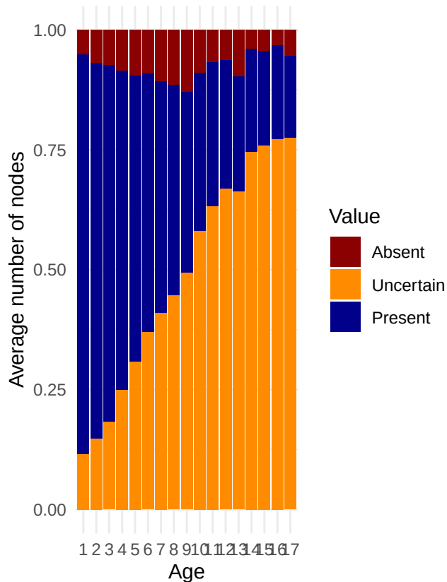
Consensus
