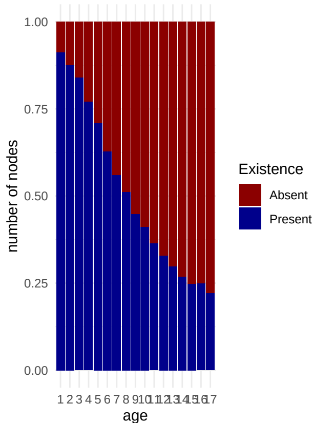
MCC
