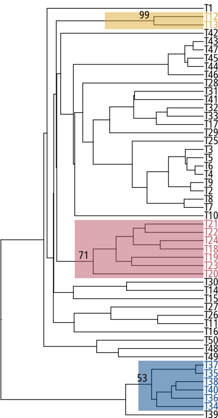
True tree
