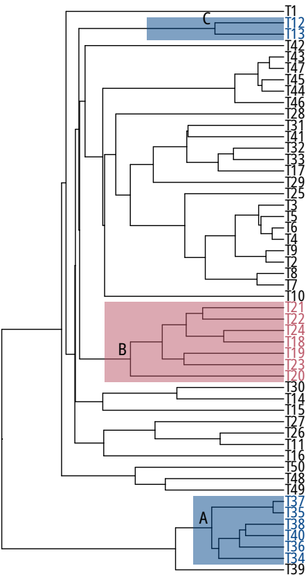
True tree
