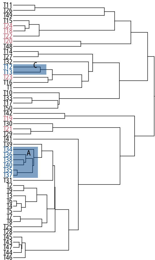
MCC tree
