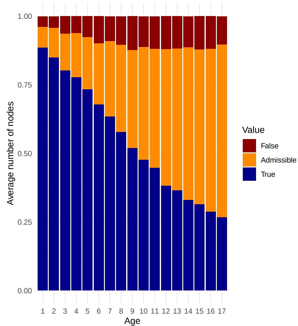
Consensus
